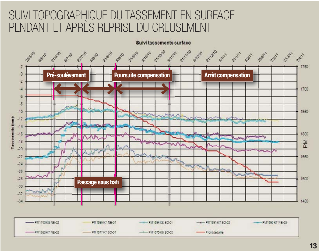
13- Topographic monitoring of surface subsidence during and after resumption of excavation.
